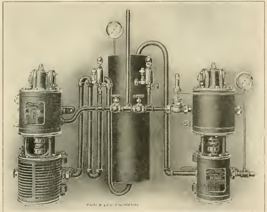
ARRANGEMENT OF PUMPS FOR PUMPING A HIGH PRESSURE OF AIR WITH LOW STEAM PRESSURE FOR SHOP PURPOSES.
